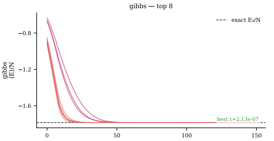
Best 8 convergence curves — j1j2_1d/j1j2_1d_20260527_170753/N12_J20.75 ( |E/N| \leq 10.0 ) Colour = learning rate
