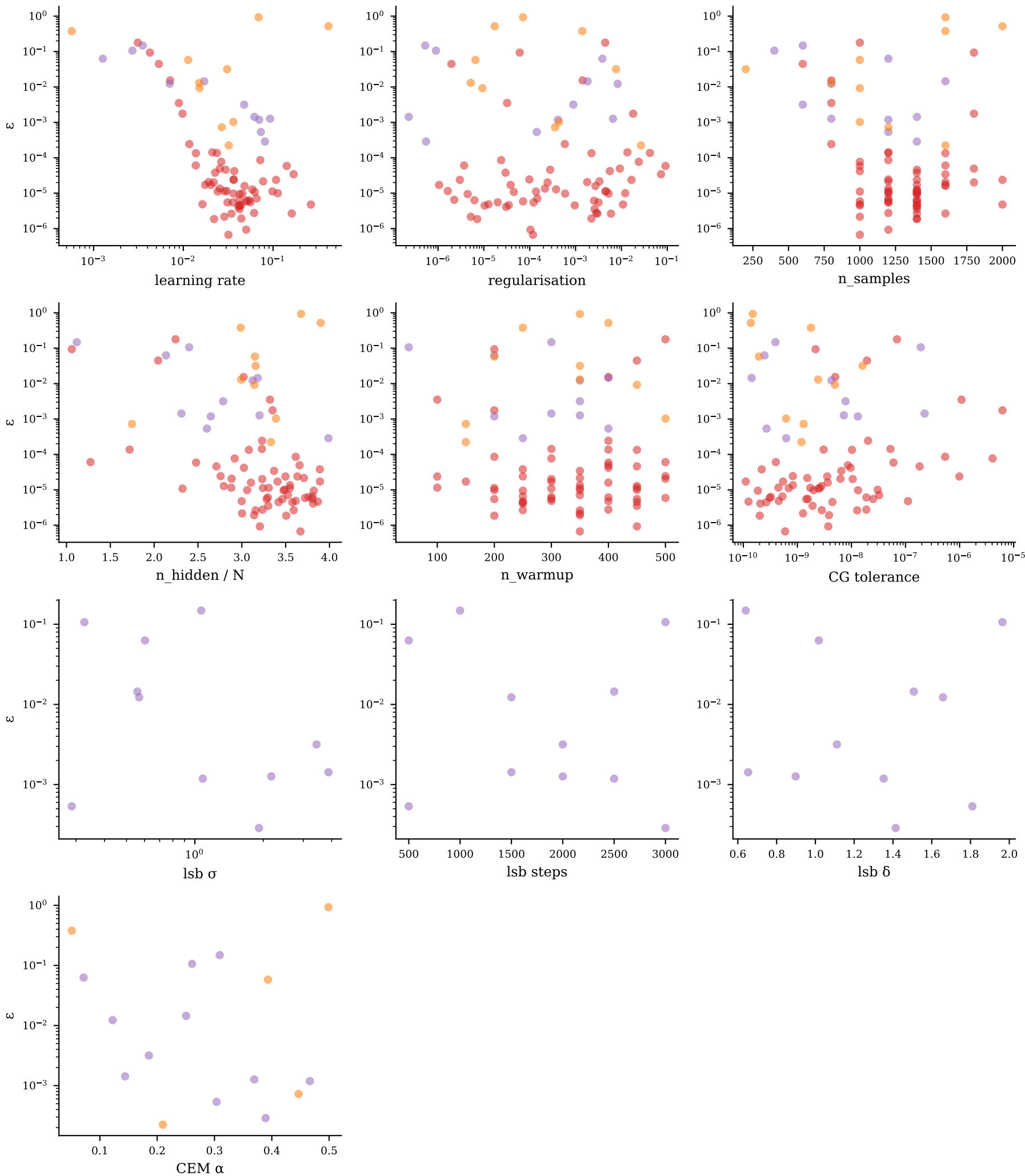
Hyperparameter sensitivity — j1j2_1d/j1j2_1d_20260527_170753/N16_J20.25
