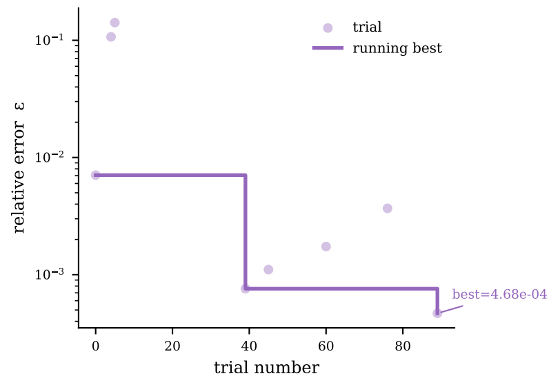
lsb (8 trials)
