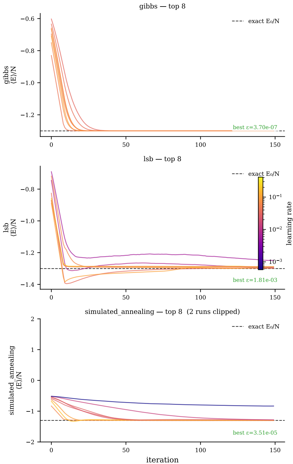
Best 8 convergence curves — j1j2_1d/j1j2_1d_20260527_170753/N8_J20.25 ( |E/N| \leq 10.0 ) Colour = learning rate
