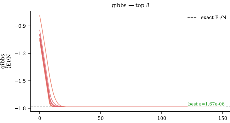
Best 8 convergence curves — j1j2_1d/j1j2_1d_20260527_170753/N8_J20.75 ( |E/N| \leq 10.0 ) Colour = learning rate
