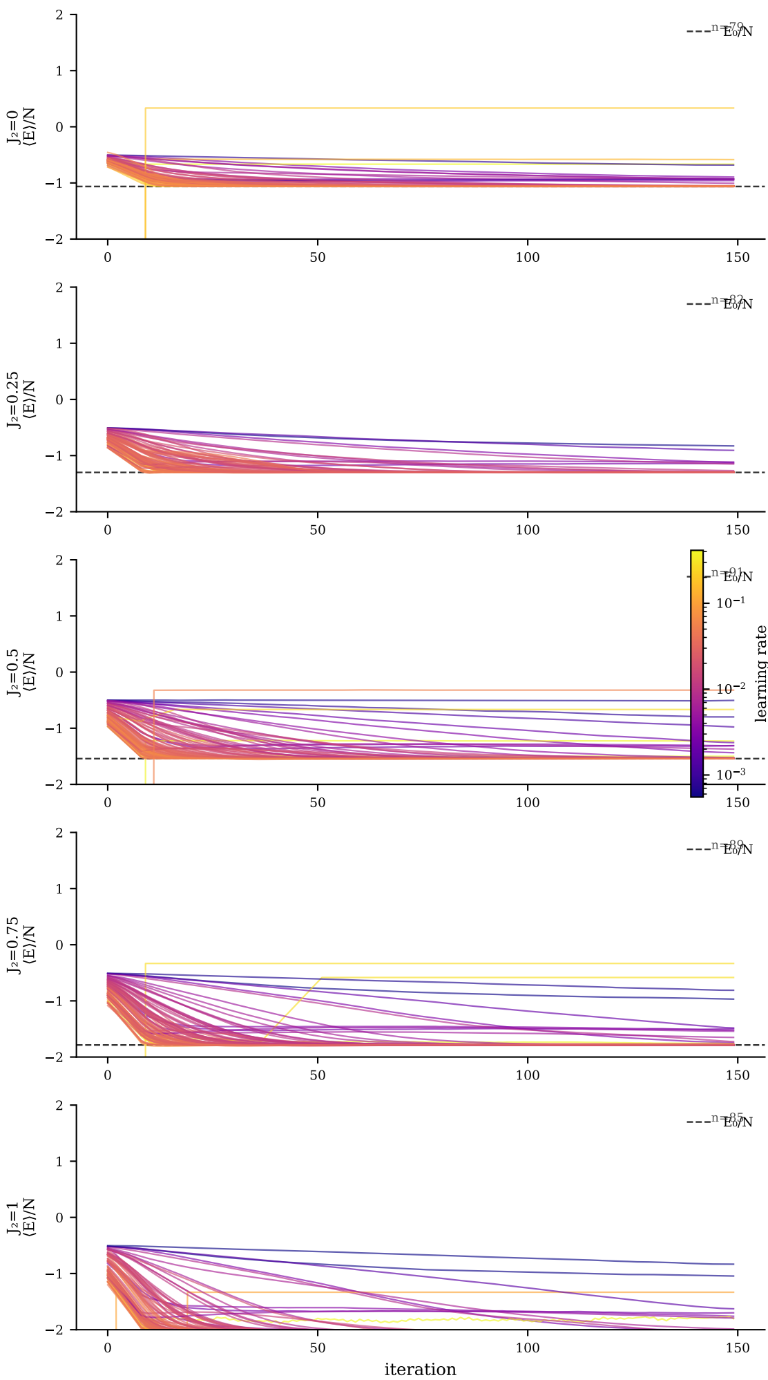
Convergence per J_2 - j_1 j_2\_1d/j_1 j_2\_1d\_20260527\_170753/N12 Each line = one trial · colour = learning rate
