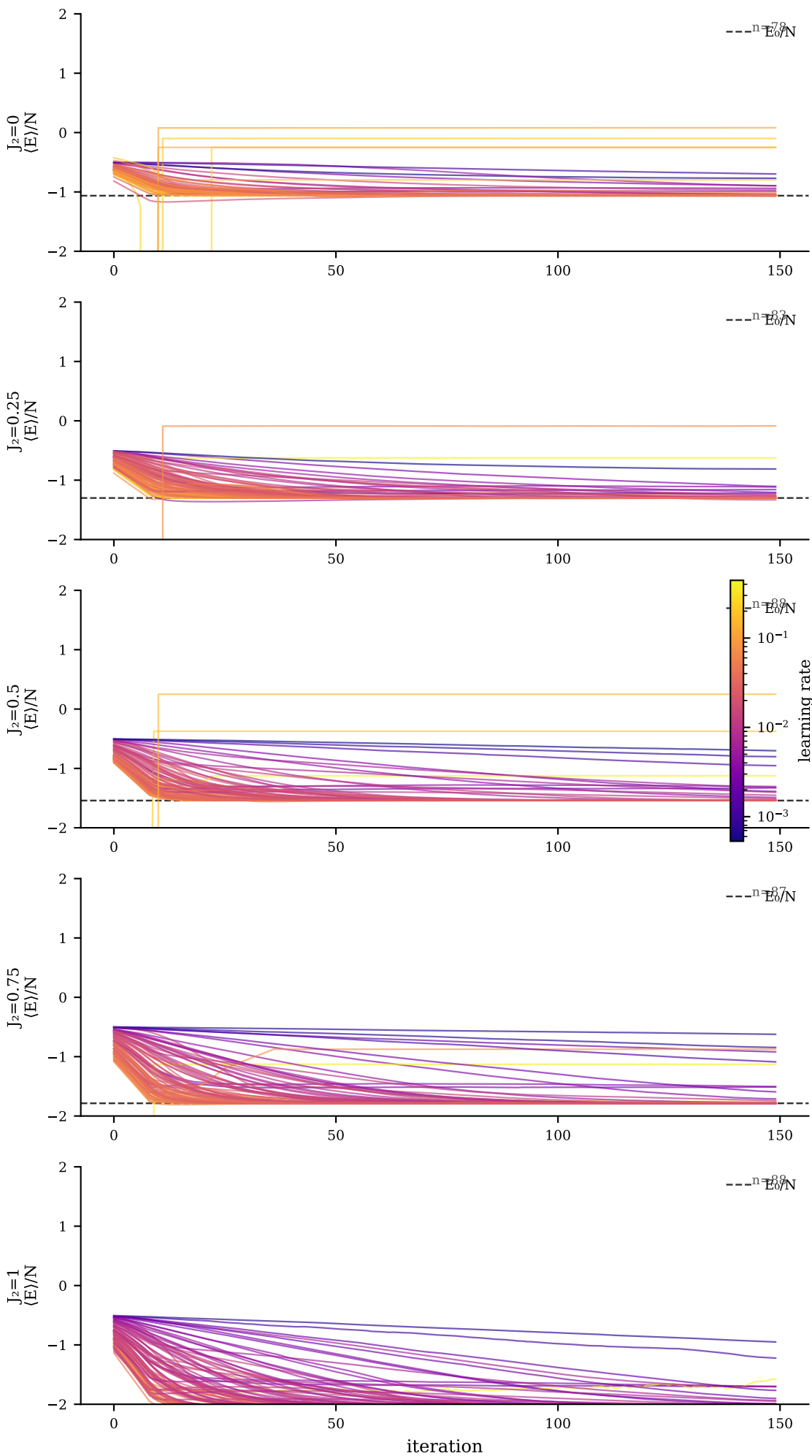
Convergence per J_2 - j1j2\_1d/j1j2\_1d\_20260527\_170753/N16 Each line = one trial · colour = learning rate
