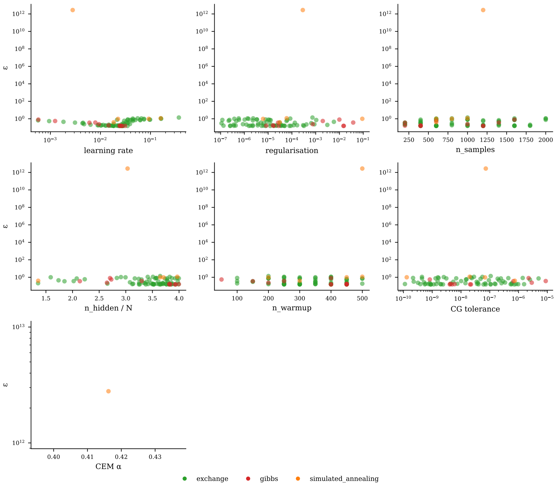
Hyperparameter sensitivity — N16_J20.9
