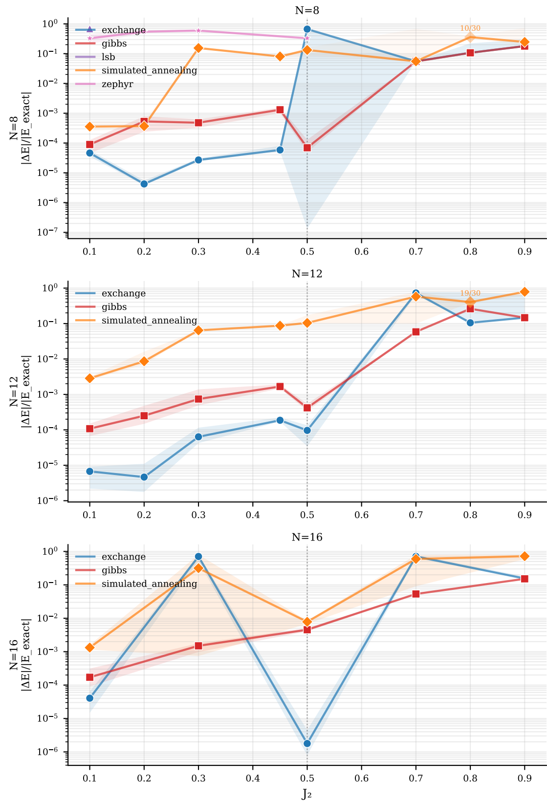
Relative energy error vs J_2 — heisenberg_j1j2_1d (isotropic Heisenberg)
