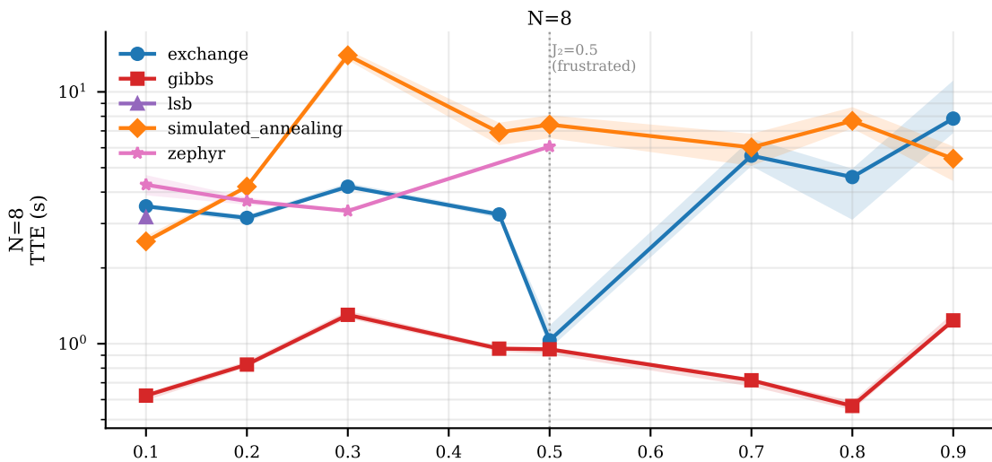
Time-to-Convergence vs J_2 (heisenberg_j1j2_1d (isotropic Heisenberg)) rolling std < 1.0\% \cdot |E_{\text{exact}}| , window=20
