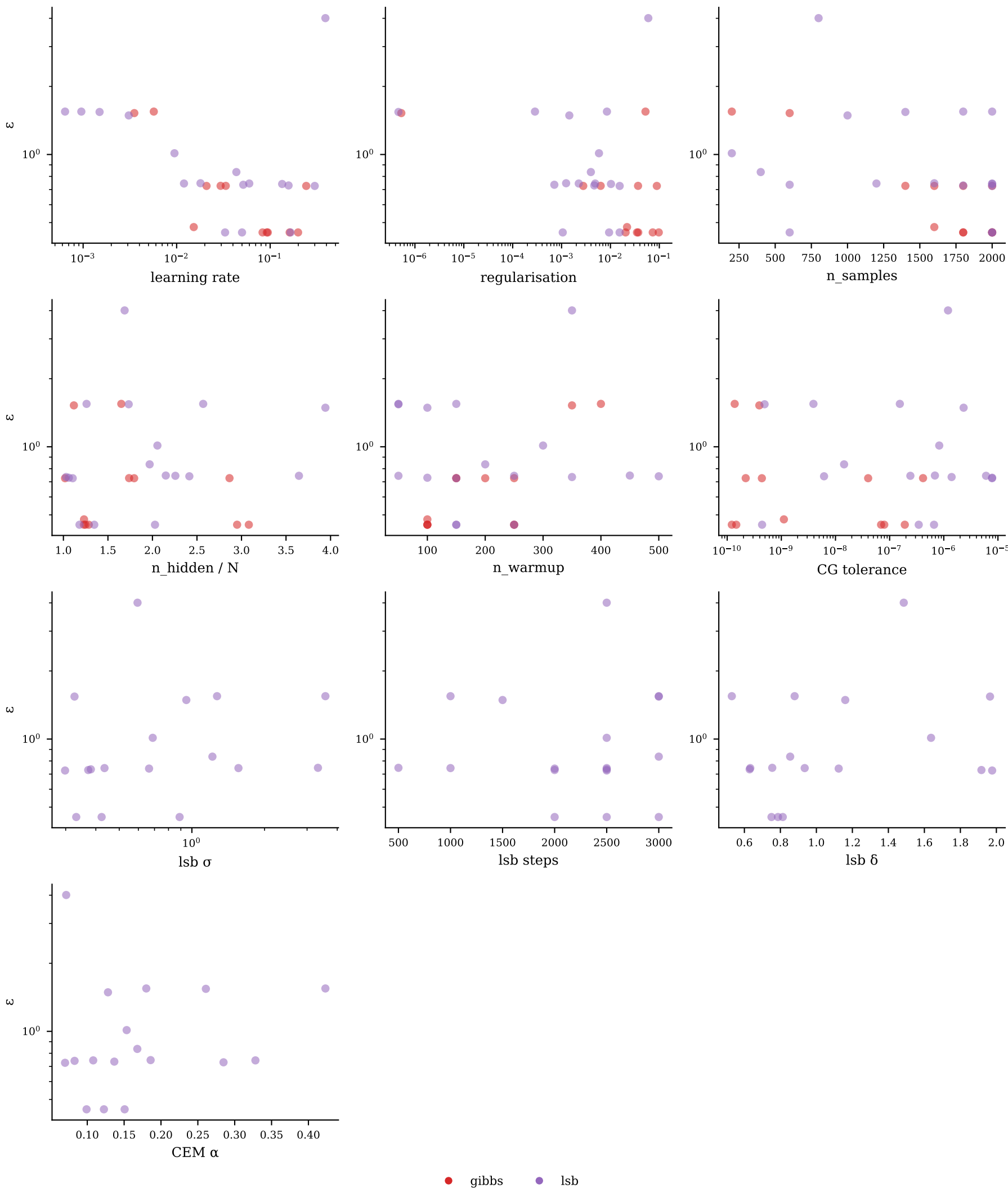
Hyperparameter sensitivity — heisenberg_xxz_1d/heisenberg_xxz_1d_20260527_150056/N8_delta1.0
