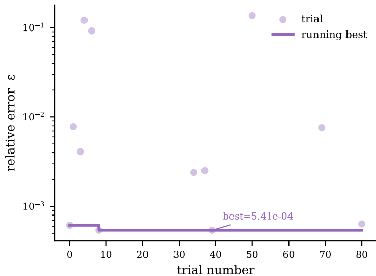
lsb (12 trials)
