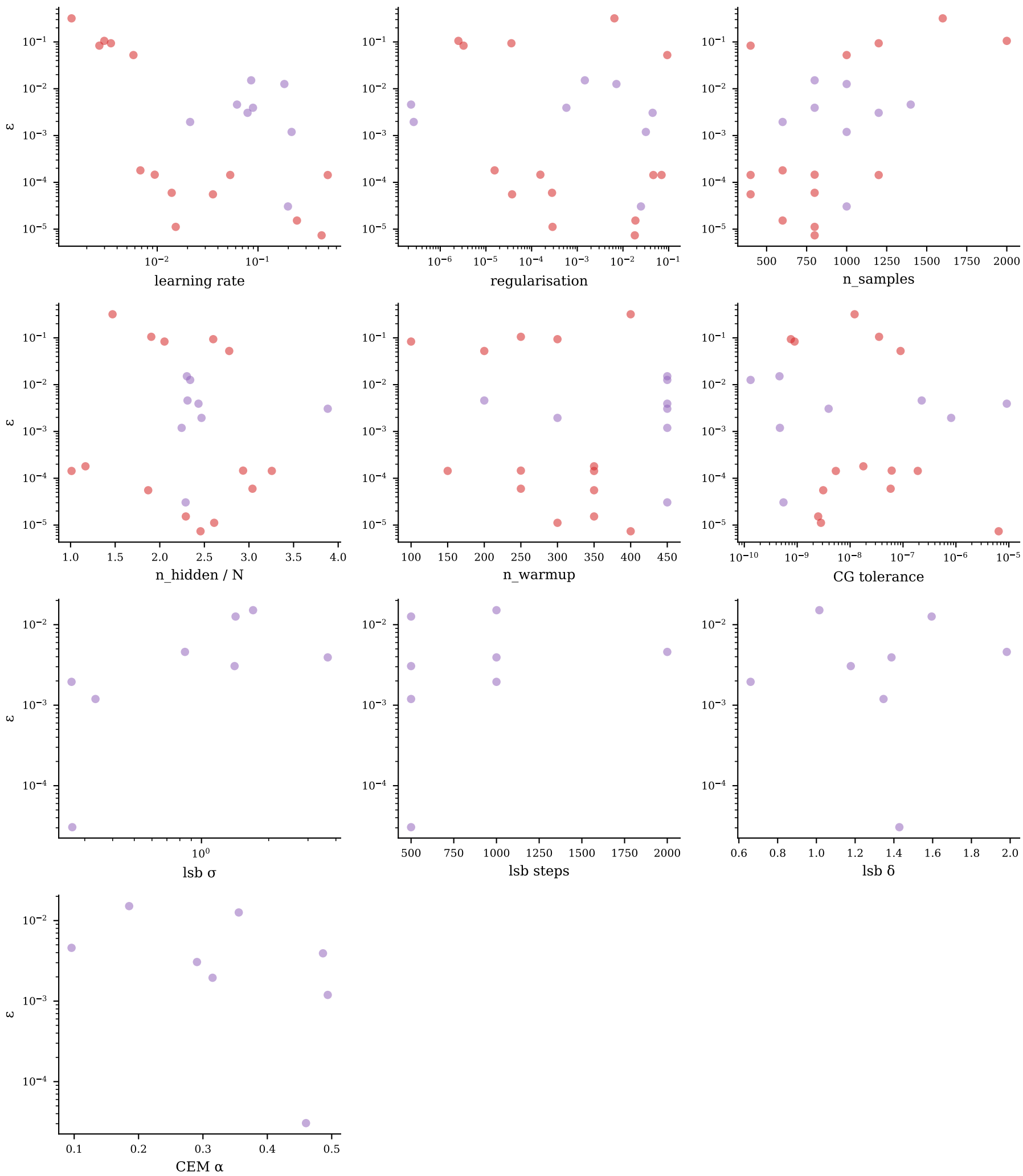
Hyperparameter sensitivity — j1j2_1d/j1j2_gibbs_lsb_v1
