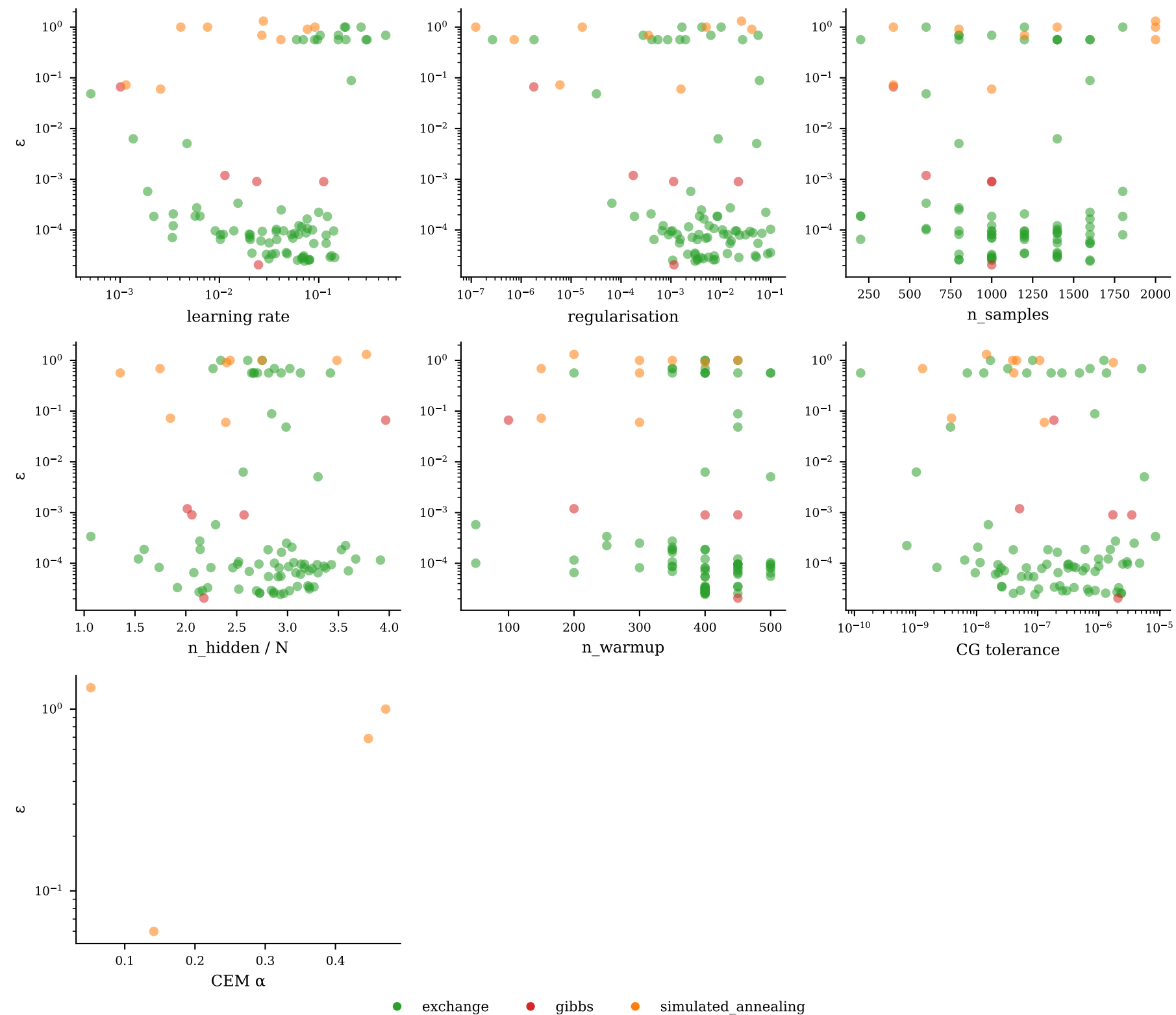
Hyperparameter sensitivity — heisenberg_j1j2_1d/heisenberg_j1j2_1d_20260528_124115/N8_J20.3
