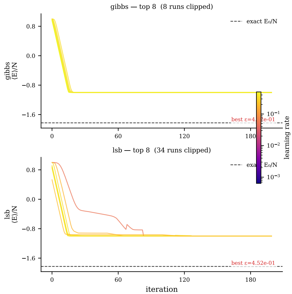
Best 8 convergence curves — heisenberg_j1j2_1d/j1j2_gibbs_lsb_v1/N8_J20.0 ( |E/N| \leq 10.0 ) Colour = learning rate
