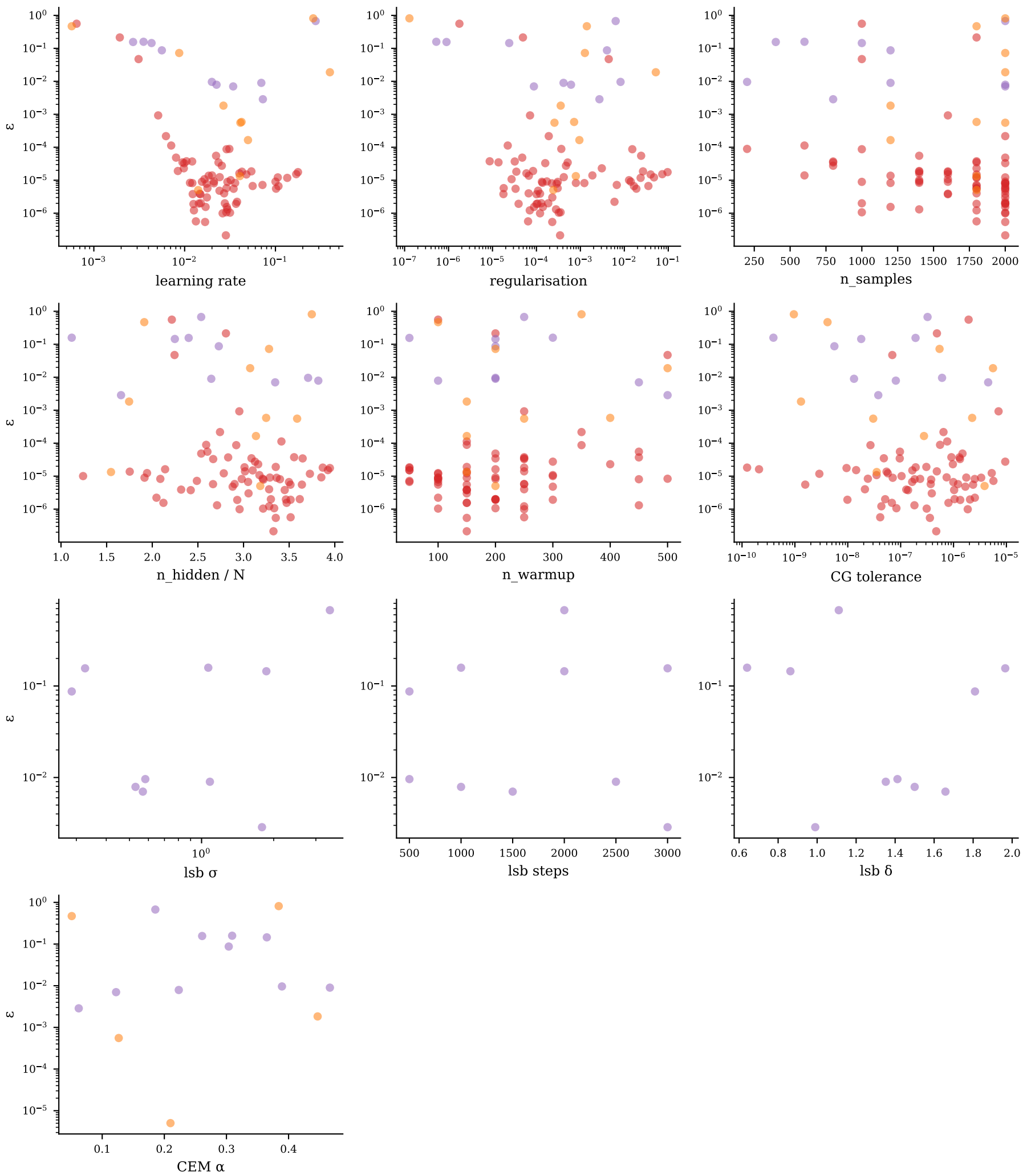
Hyperparameter sensitivity — j1j2_1d/j1j2_1d_20260527_170753/N12_J20.75
