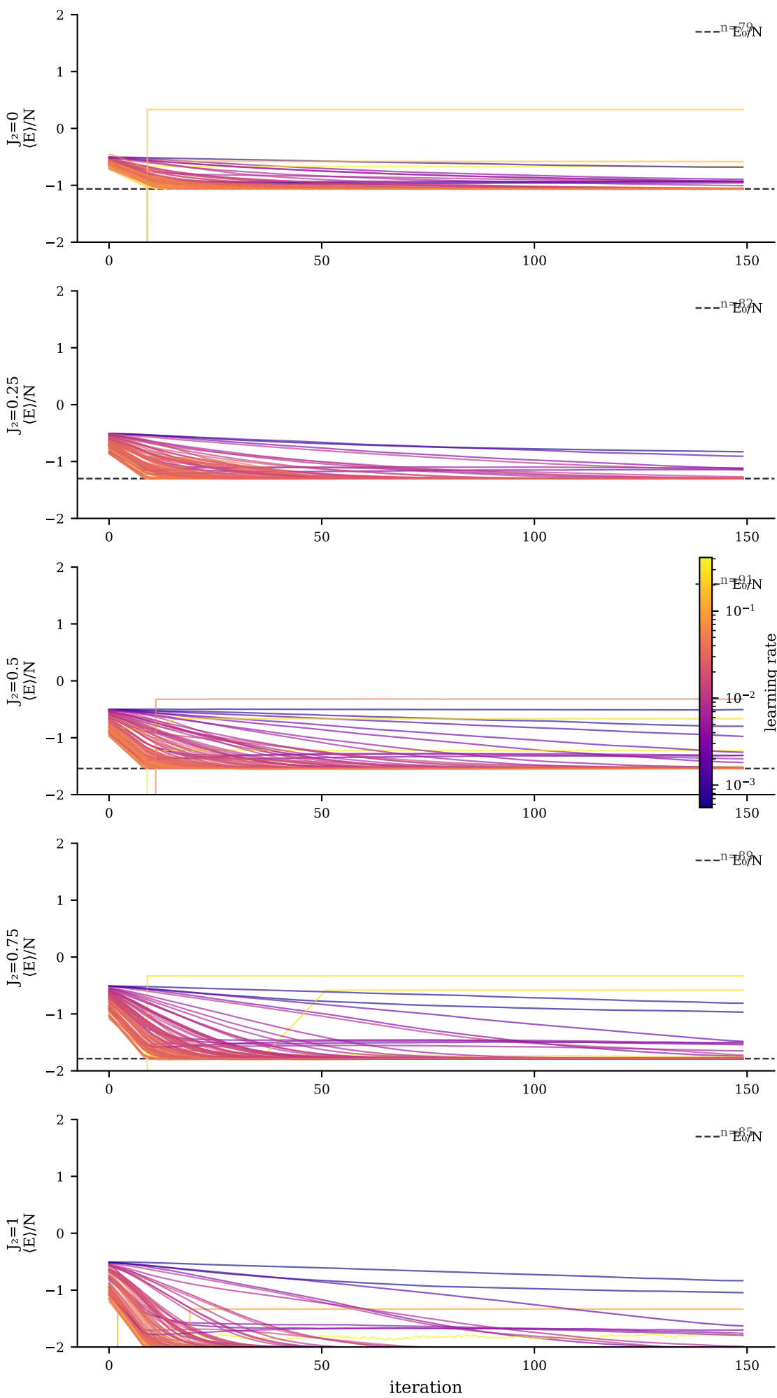
Convergence per J_2 - j_1 j_2\_1d\_20260527\_170753/N12 Each line = one trial · colour = learning rate
