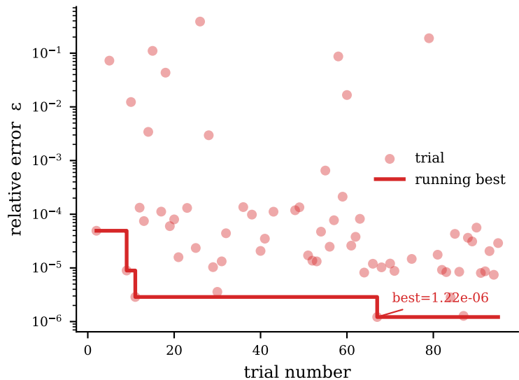
gibbs (65 trials)
