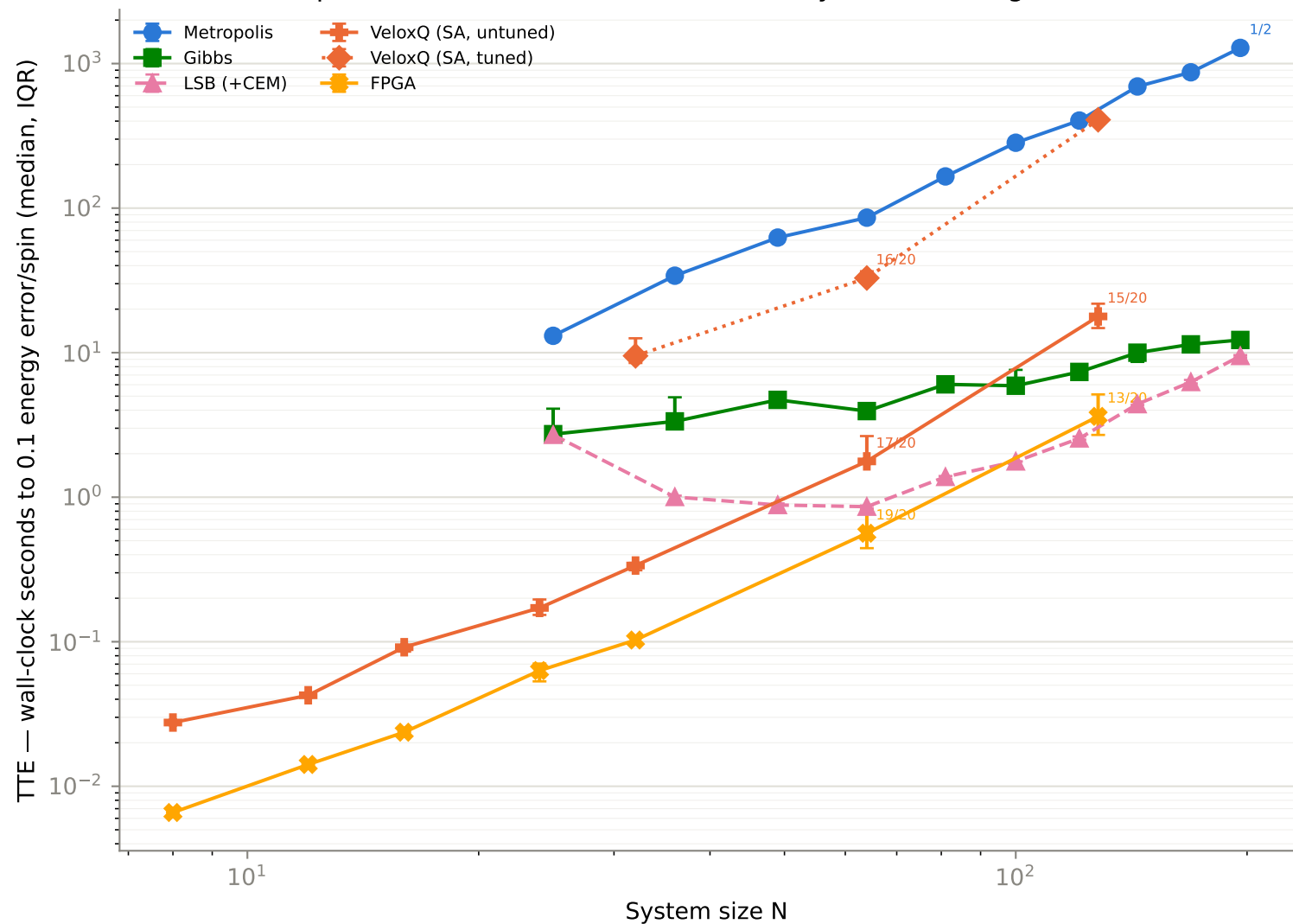
Time-to-epsilon vs. N (D-Wave QPU shown only where timing was recorded)
