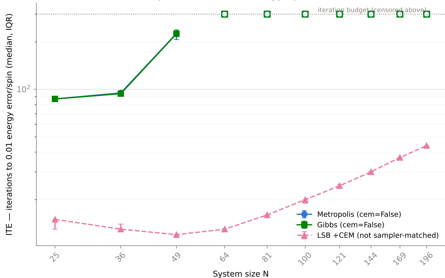
Iterations-to-epsilon vs. system size TFIM 1D, critical point h=1.0 , matched hyperparameters, no best-of
