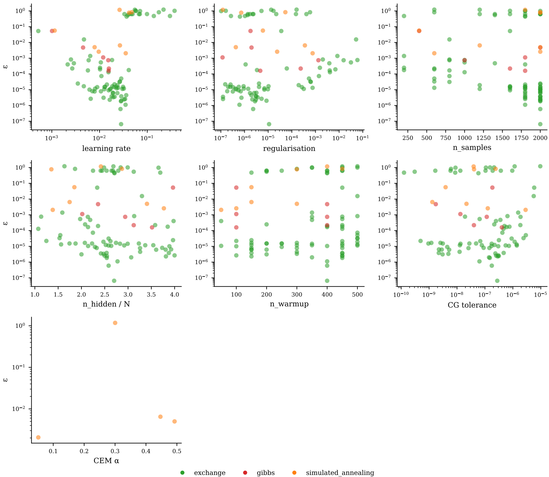
Hyperparameter sensitivity — heisenberg_1j2_1d/heisenberg_1j2_1d_20260528_124115/N12_J20.1
