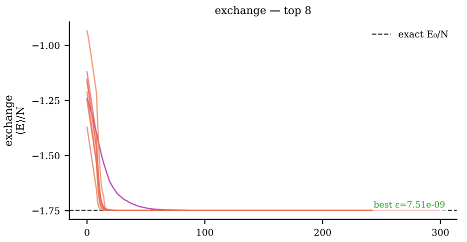
Best 8 convergence curves — heisenberg_j1j2_1d/heisenberg_j1j2_1d_20260528_124115/N8_J20.1 ( |E/N| \leq 10.0 ) Colour = learning rate
