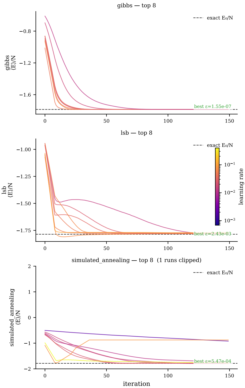
Best 8 convergence curves — j1j2_1d/j1j2_1d_20260527_170753/N16_J20.75 ( |E/N| \leq 10.0 ) Colour = learning rate
