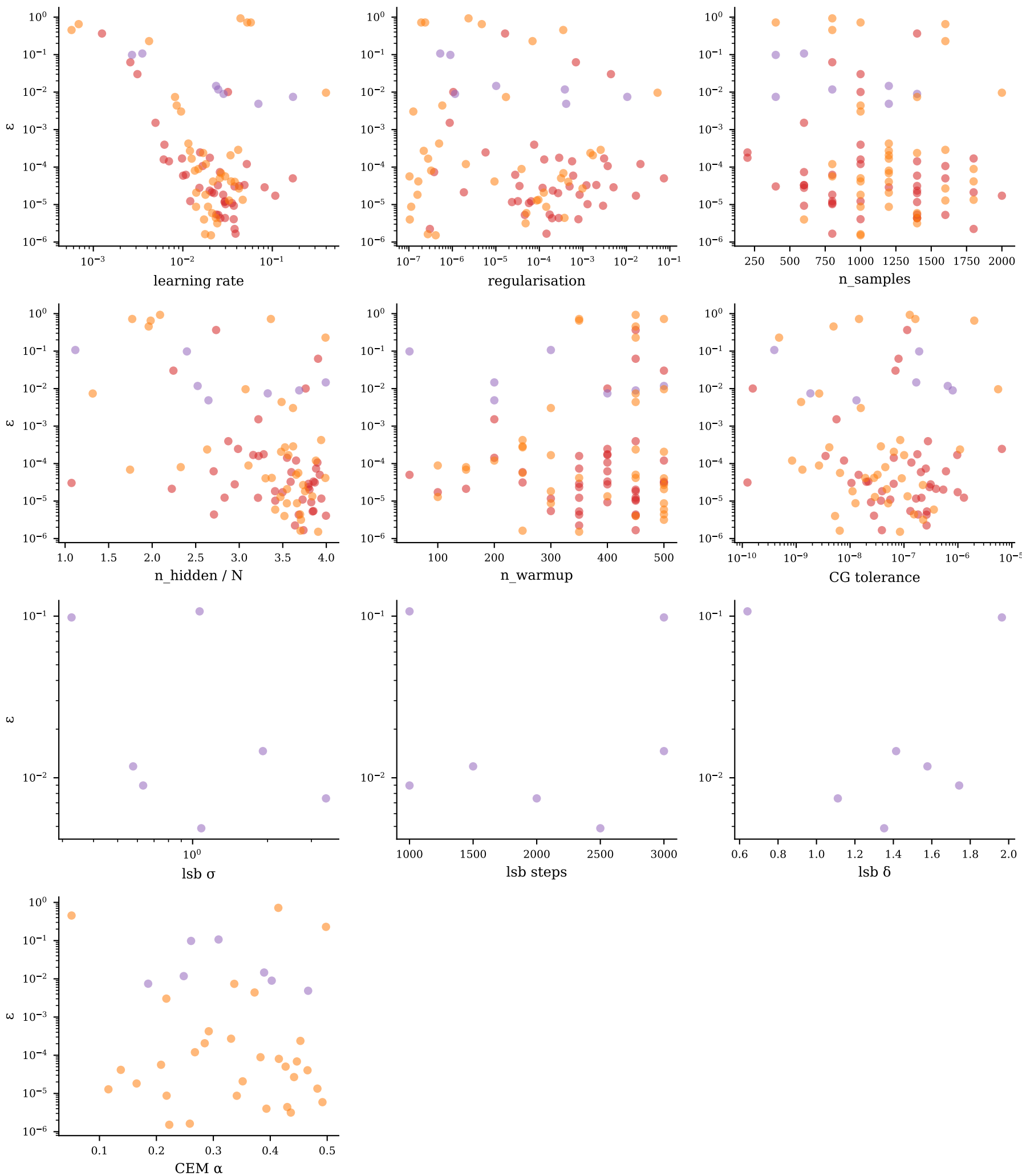
Hyperparameter sensitivity — j1j2_1d/j1j2_1d_20260527_170753/N8_J20.75
