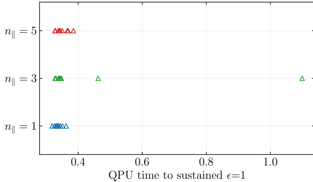
Time-to- \epsilon — events (dots), censored (open triangles), KM median (bar) with bootstrap 95
