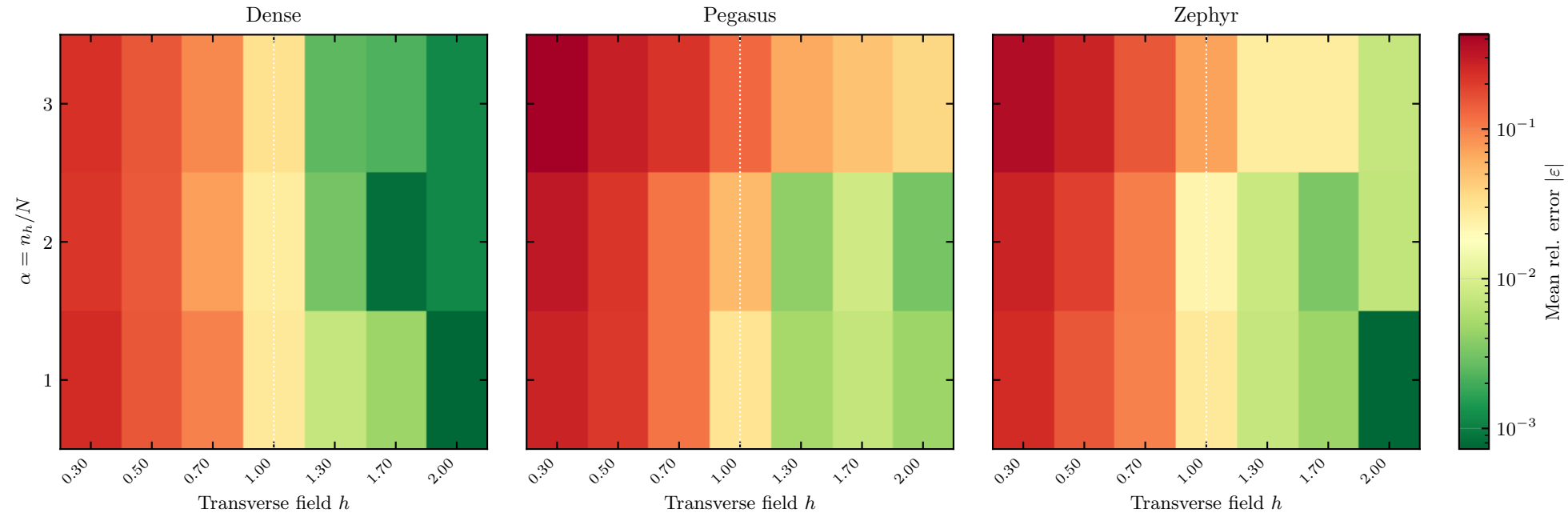
Energy error vs. (\alpha, h) — N = 8
