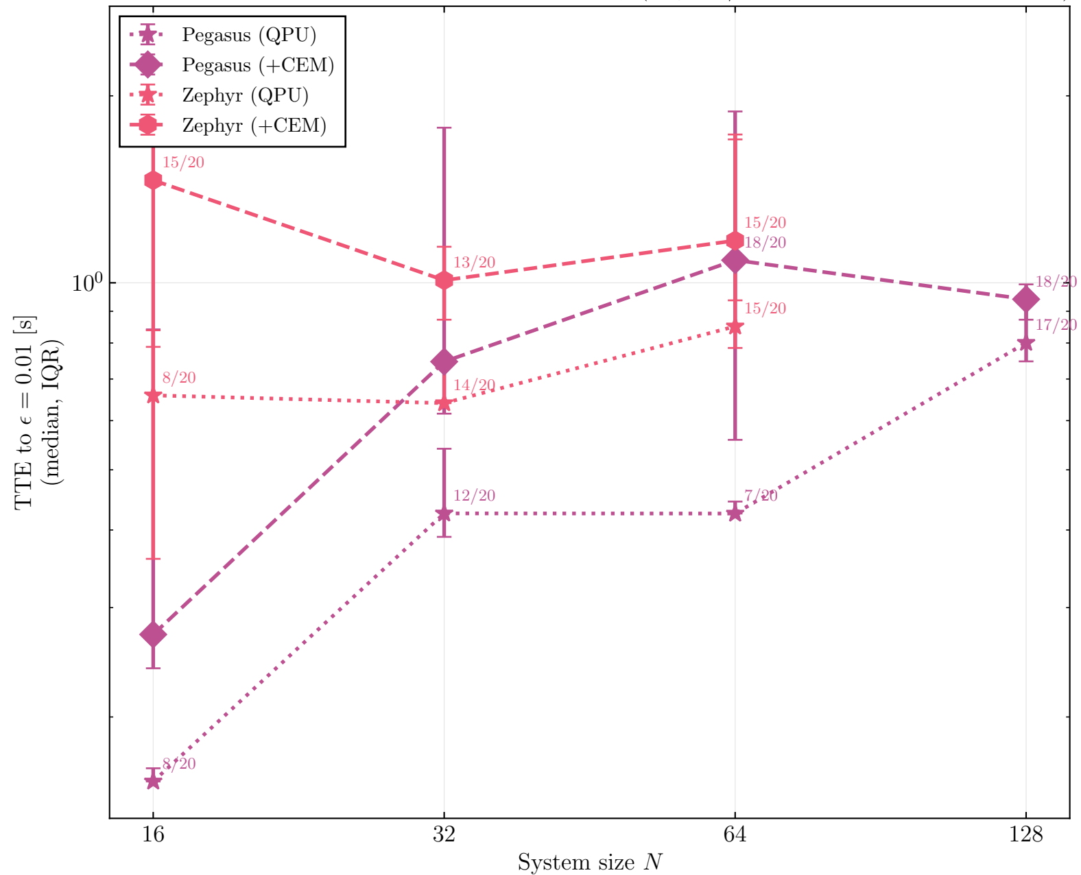
Time-to- \epsilon vs. system size N — D-Wave QPUs only (Pegasus/Zephyr, with and without CEM)
