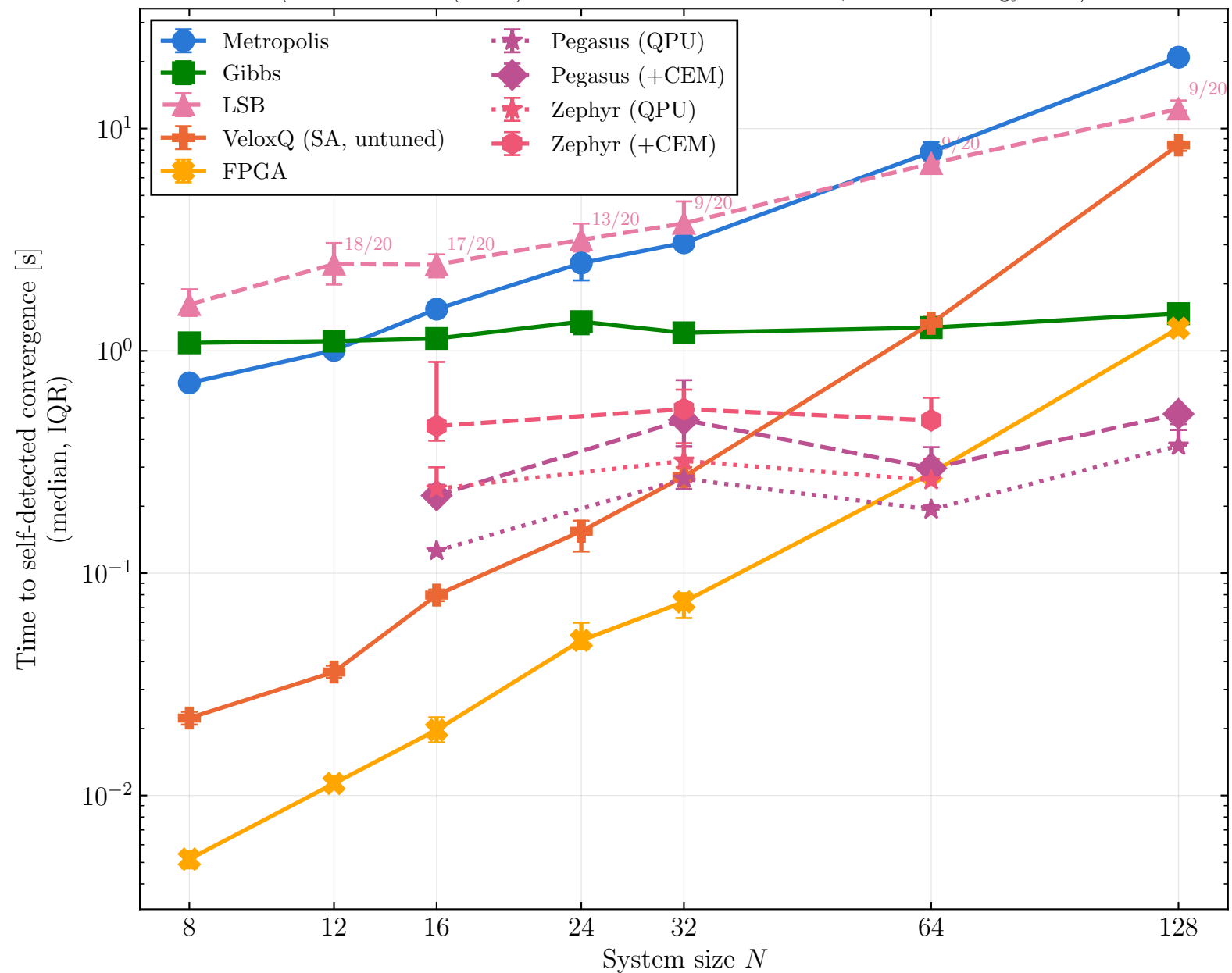
Time-to-convergence vs. system size N — all solvers (oracle-free: \text{CV}(\text{E}_{\text{loc}}) < 0.05 for 10 consecutive iters, no exact_energy used)
