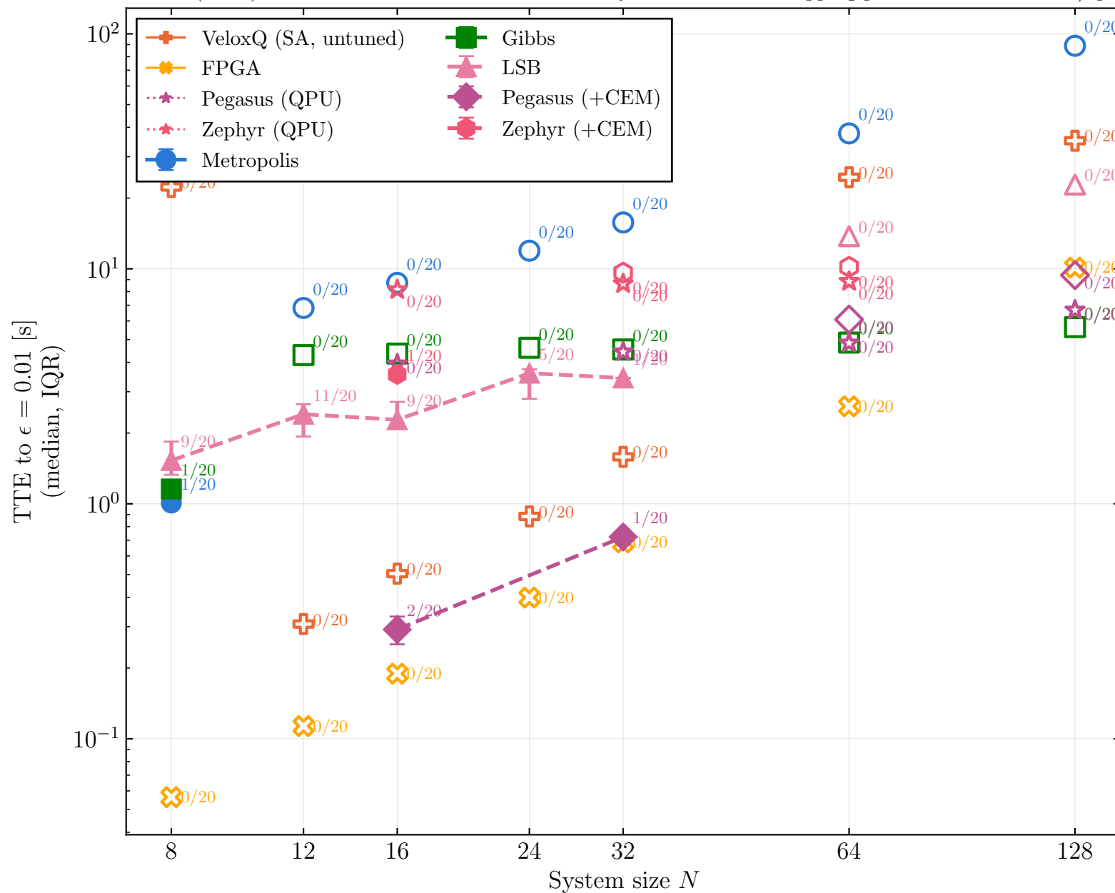
Time-to- \epsilon vs. system size N — all solvers
