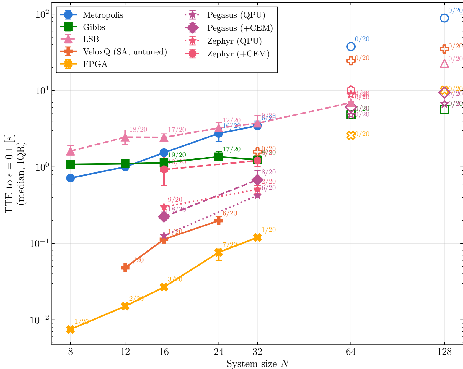
Time-to- \epsilon vs. system size N — all solvers
