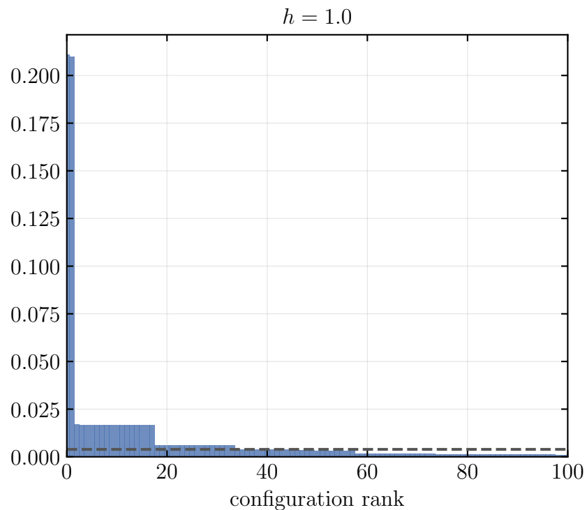
Exact |\Psi(v)|^2 distribution | TFIM 1D N = 8
