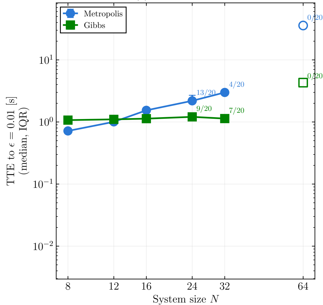
(a) Classical samplers
