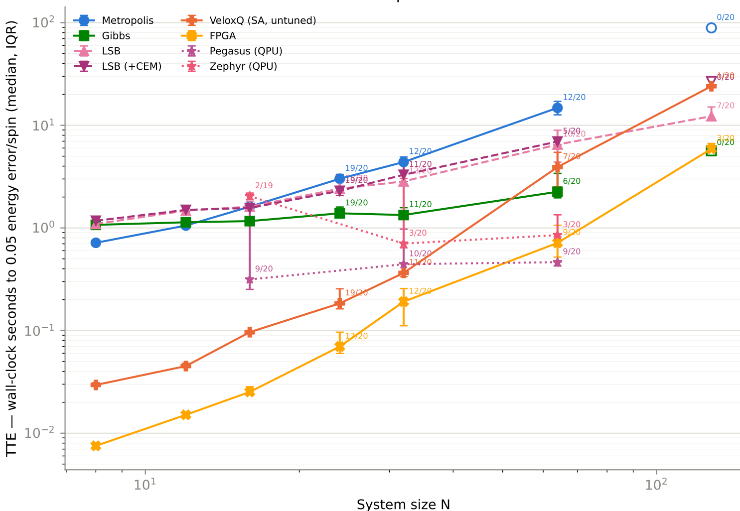
Time-to-epsilon vs. N
