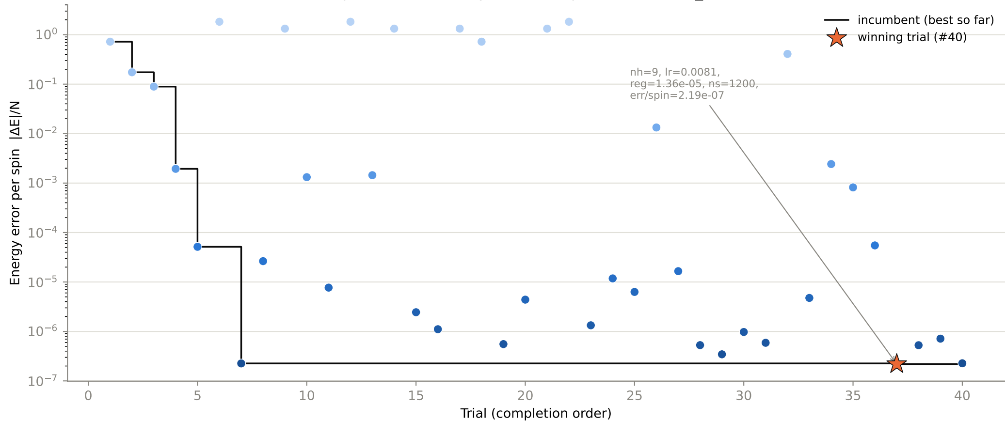
Optimization history — 40 completed trials, N8_J20.0
