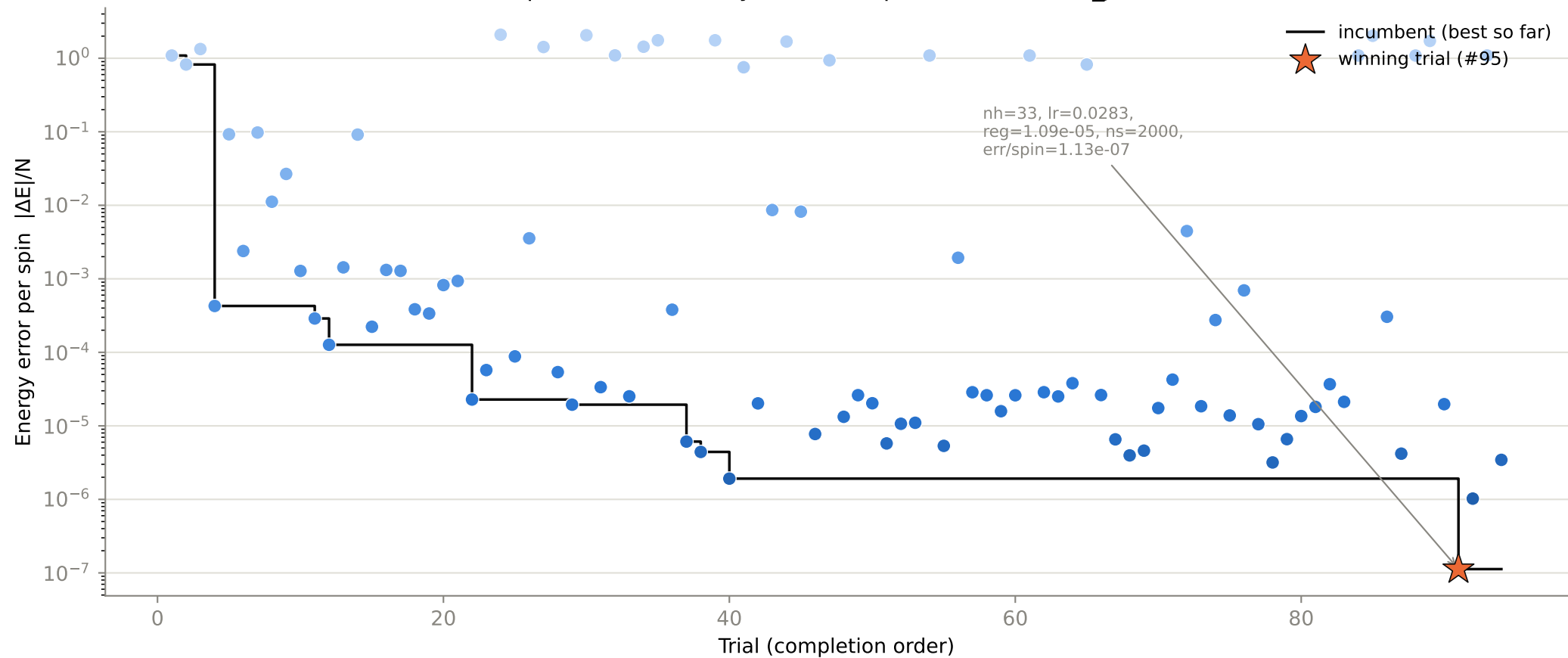
Optimization history — 94 completed trials, N12_J20.1
