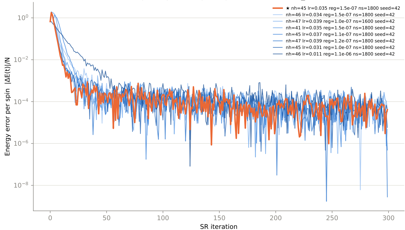
Convergence per config — top 8 of 95 trials, N12_J20.2
