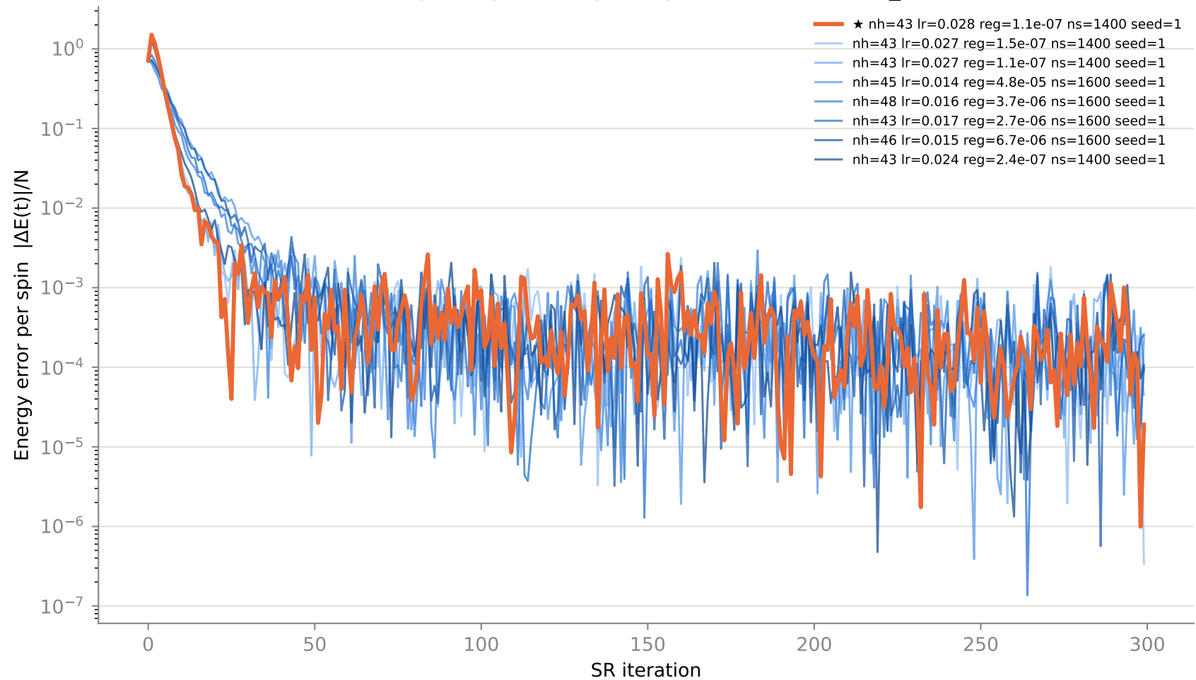
Convergence per config — top 8 of 91 trials, N12_J20.3
