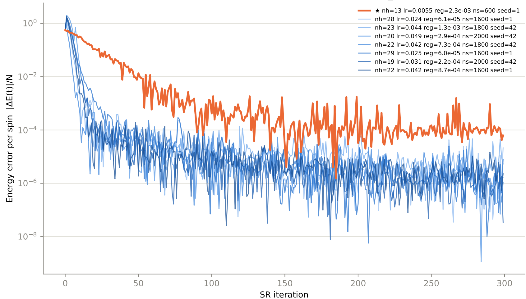
Convergence per config — top 8 of 93 trials, N8_J20.1
