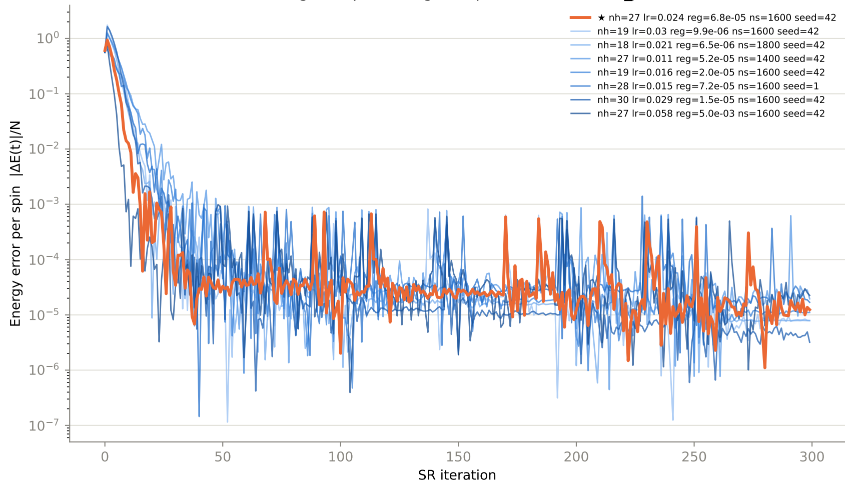
Convergence per config — top 8 of 96 trials, N8_J20.2
