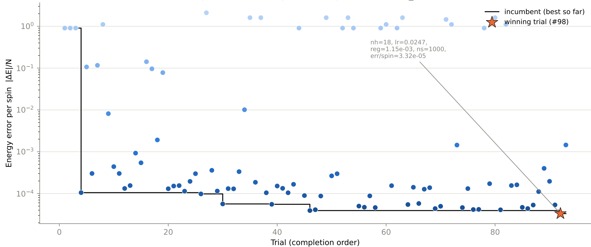
Optimization history — 93 completed trials, N8_J20.3
