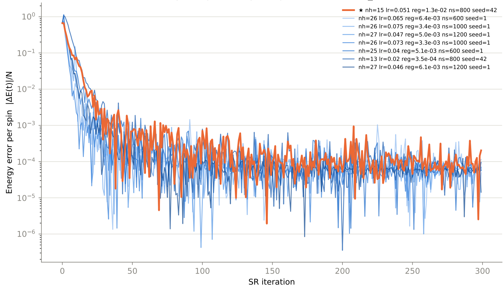
Convergence per config — top 8 of 97 trials, N8_J20.45
