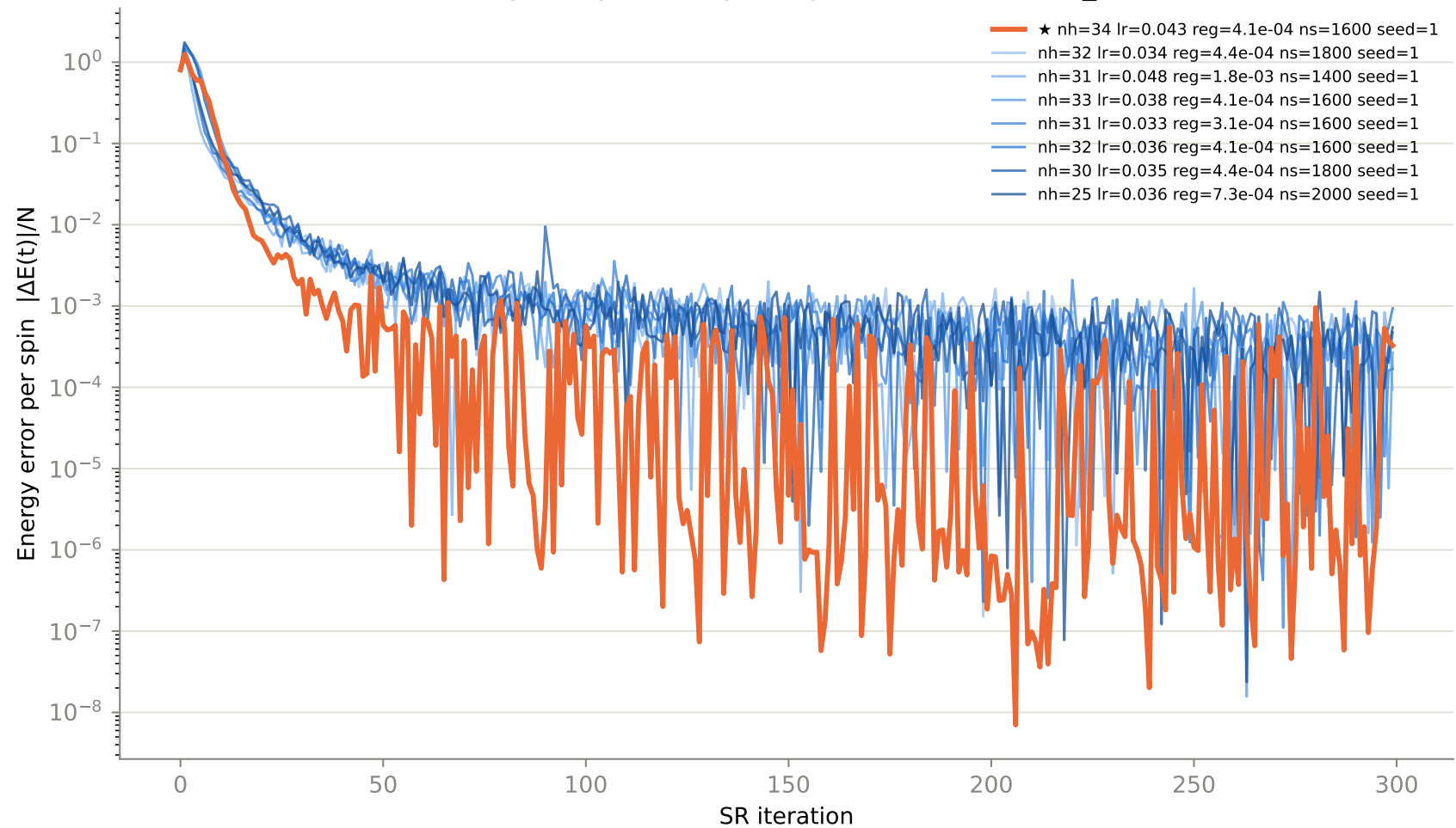
Convergence per config — top 8 of 81 trials, N12_J20.5
