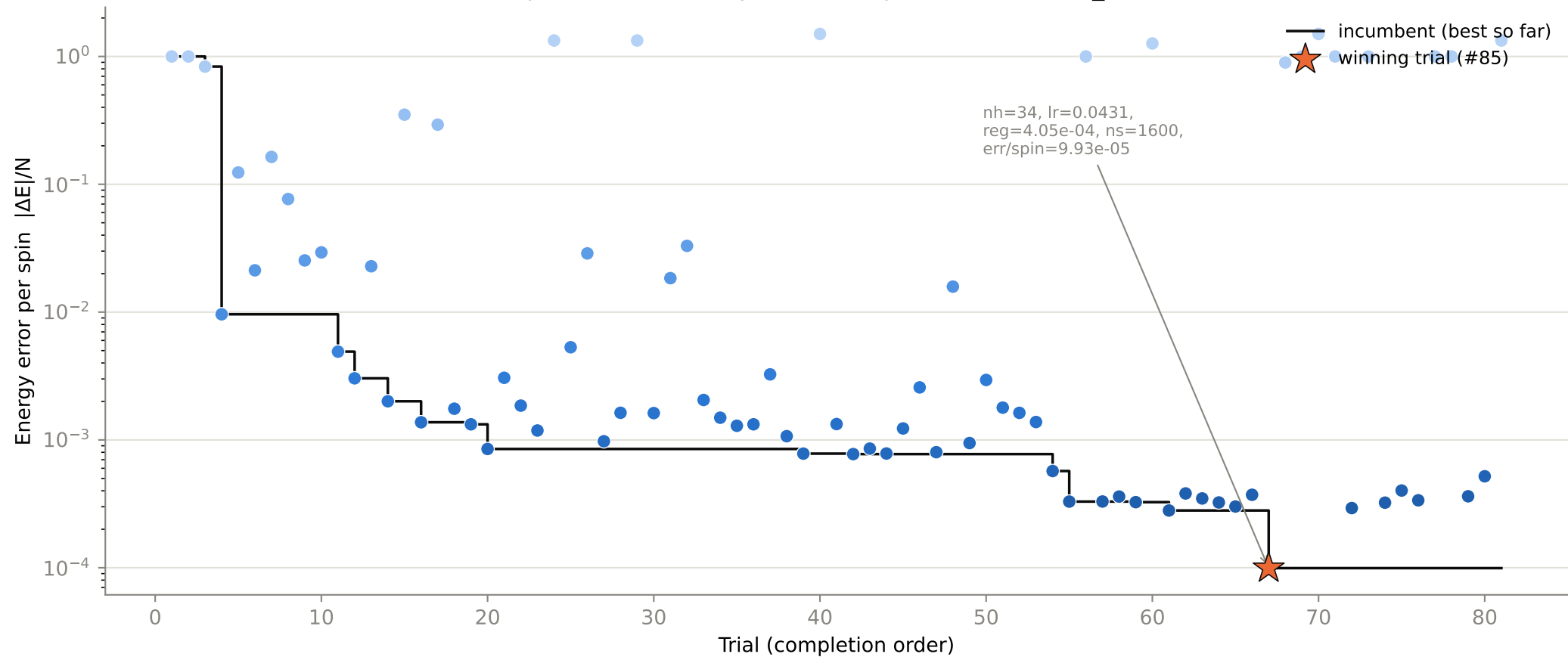
Optimization history — 81 completed trials, N12_J20.5
