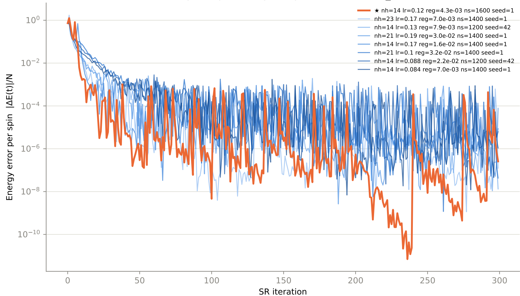
Convergence per config — top 8 of 96 trials, N8_J20.5
