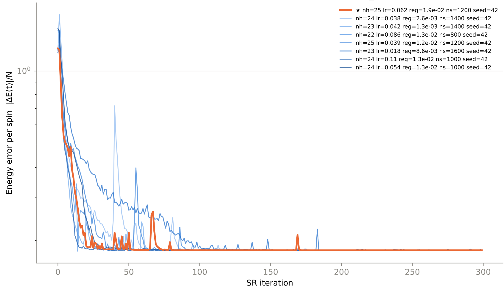
Convergence per config — top 8 of 81 trials, N8_J20.8
