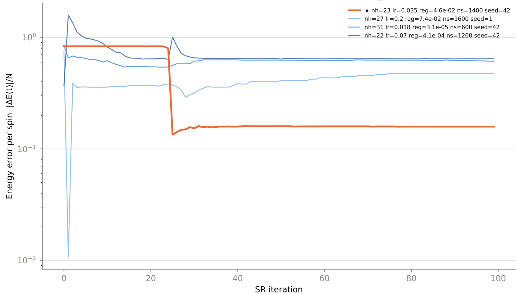
Convergence per config — top 4 of 4 trials, N8_J20.0
