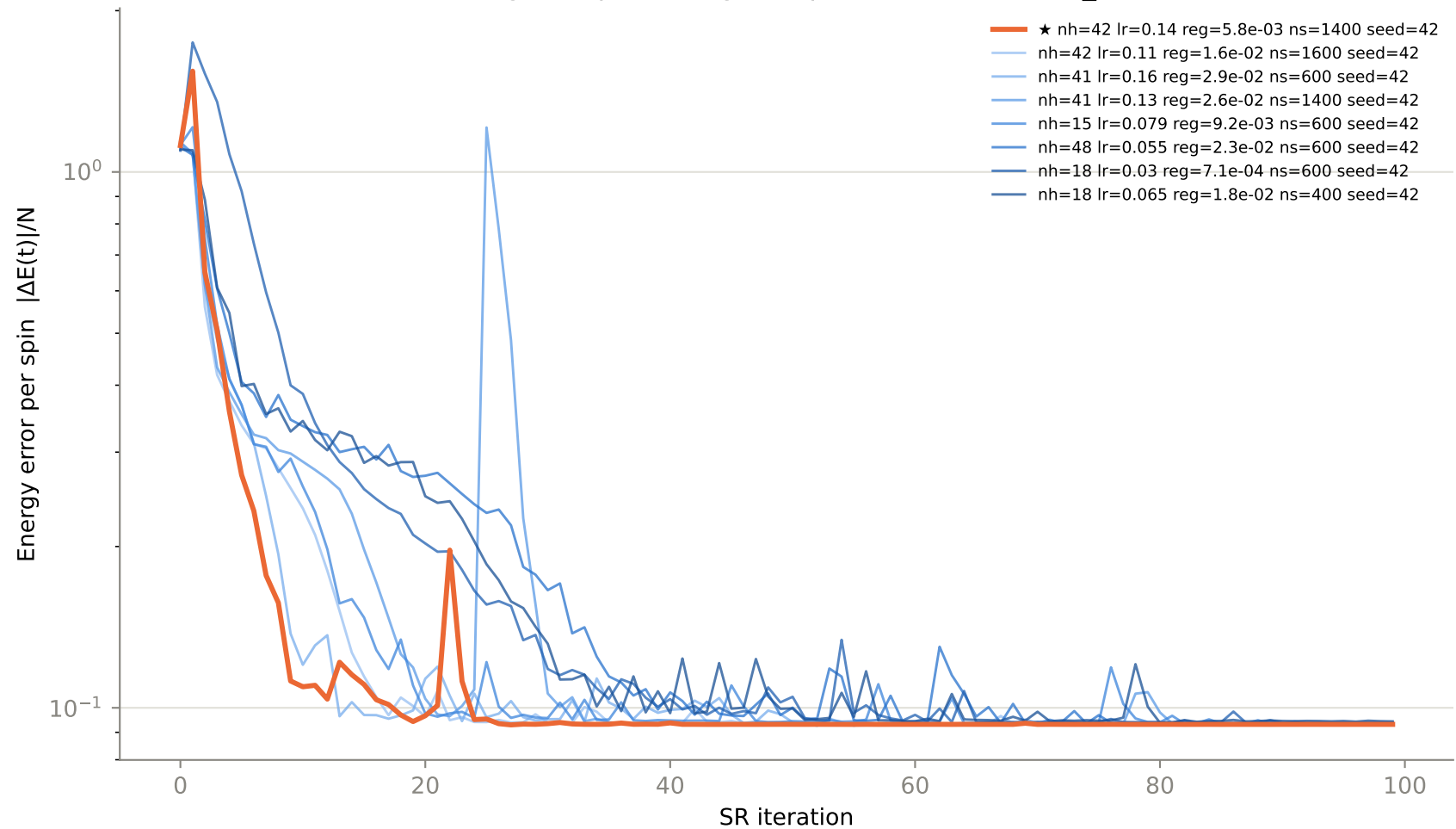
Convergence per config — top 8 of 92 trials, N12_J20.7
