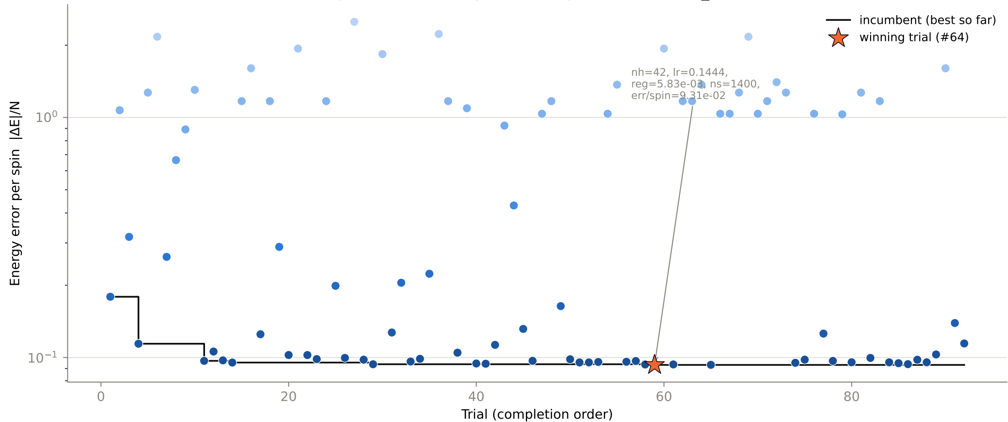
Optimization history — 92 completed trials, N12_J20.7
