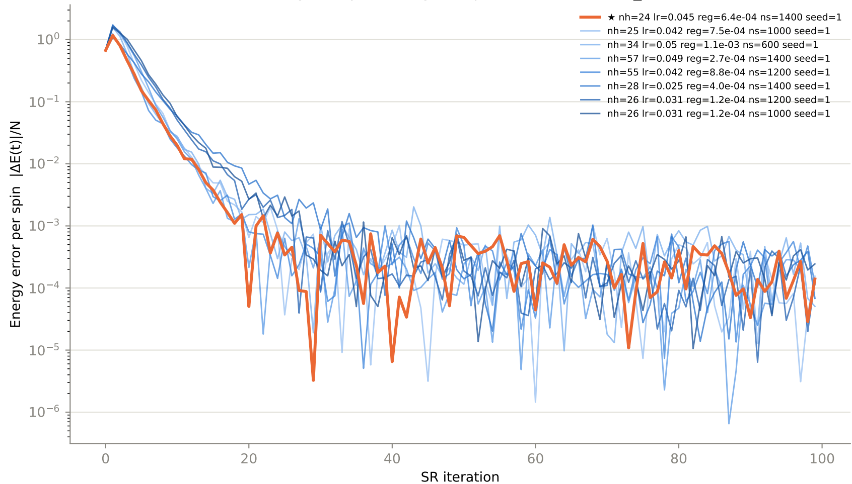
Convergence per config — top 8 of 94 trials, N16_J20.1
