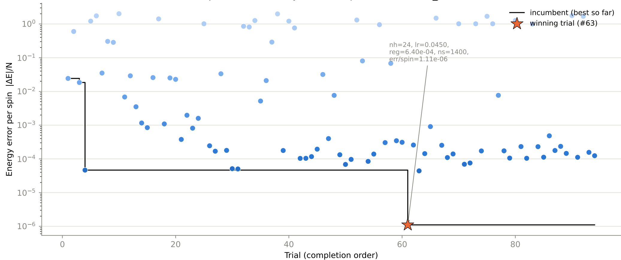
Optimization history — 94 completed trials, N16_J20.1
